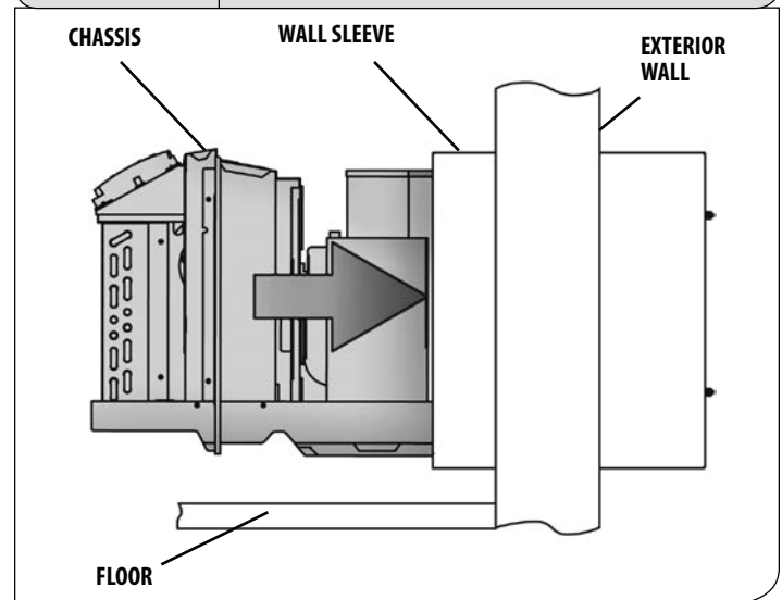
Figure 27 Chassis Installation
