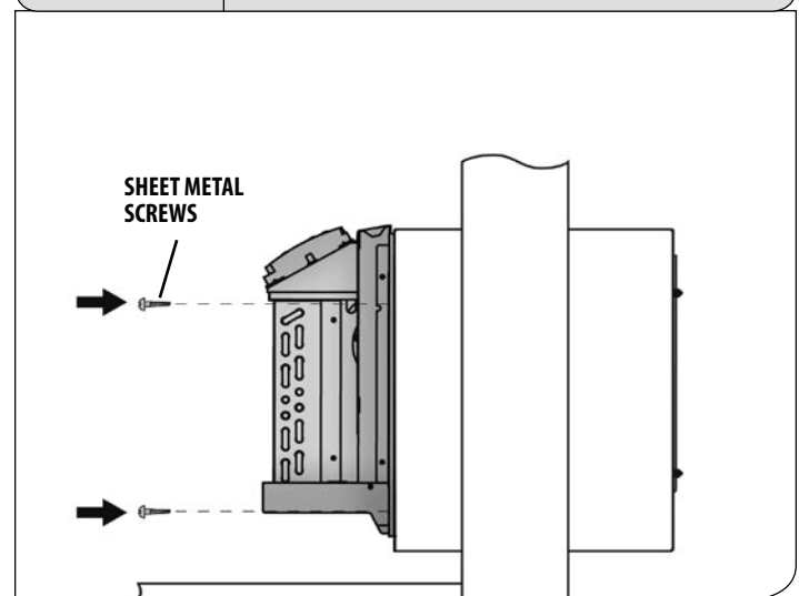
Figure 28 Chassis Installation
