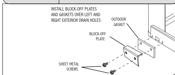
Figure 15 Block-Off Plate Installation
