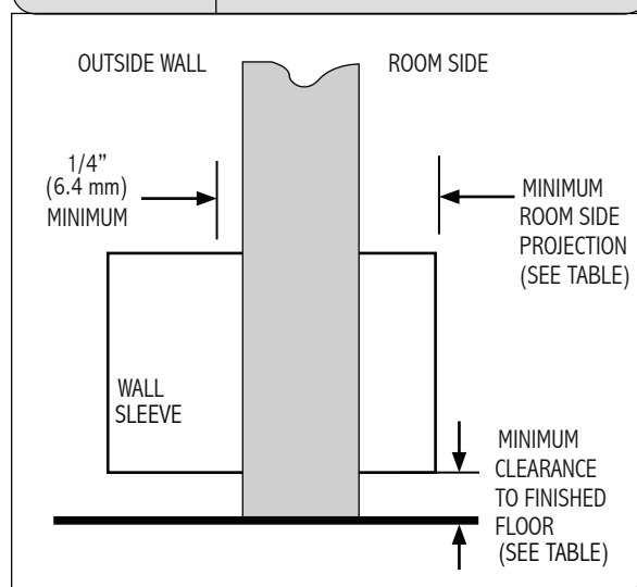
Figure 4 Minimum Clearance From Walls
