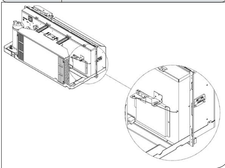
Figure 32 Fresh Air Vent
