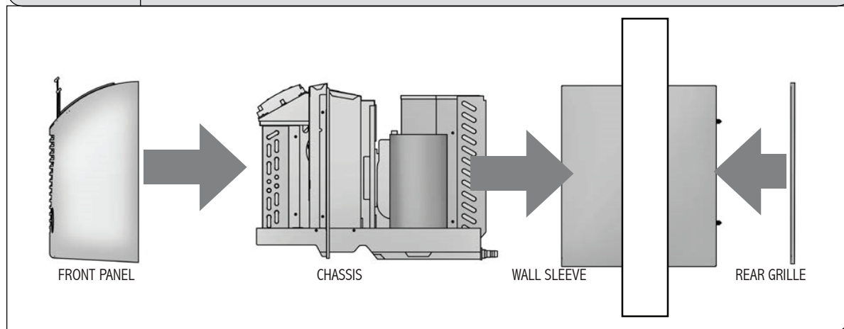
Figure 5 Main Installation Components
