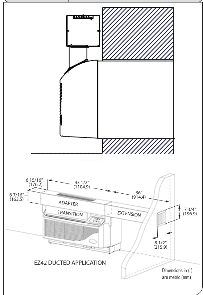
Figure 33 Lateral Duct Kit
