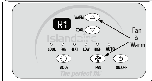
Figure 47 Display - Temp Limit Code
