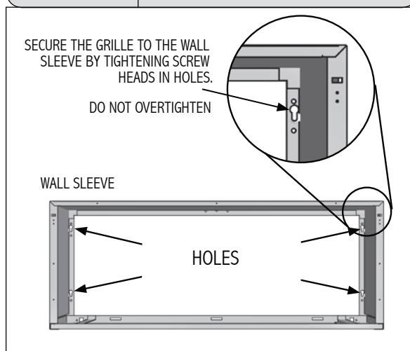
Figure 18 Standard Grille Installation
