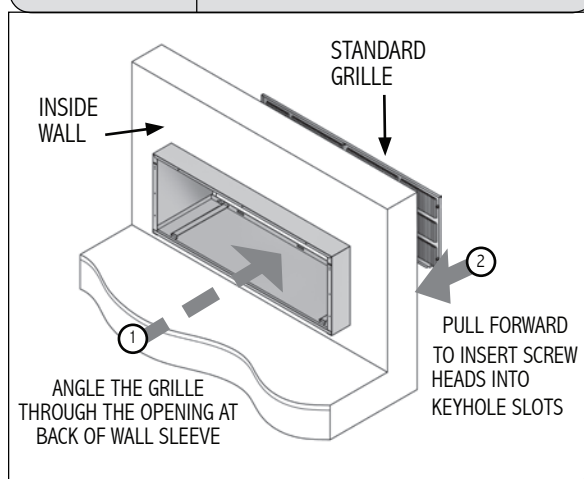
Figure 17 Standard Grille Installation
