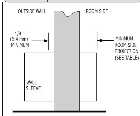
Figure 3 Minimum Clearance From Floor
