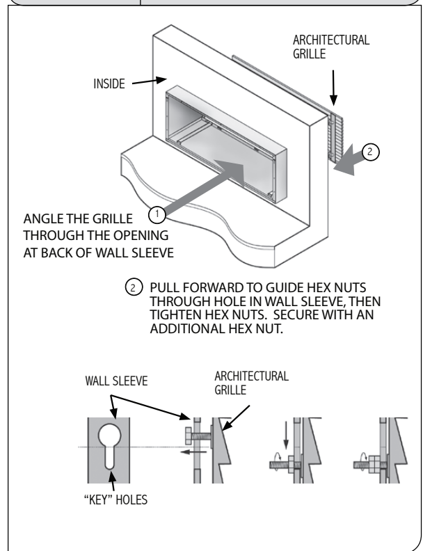
Figure 21 Arch. Rear Grille Installation
