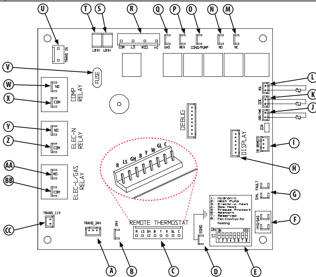
Figure 46 Control Board Physical Features
