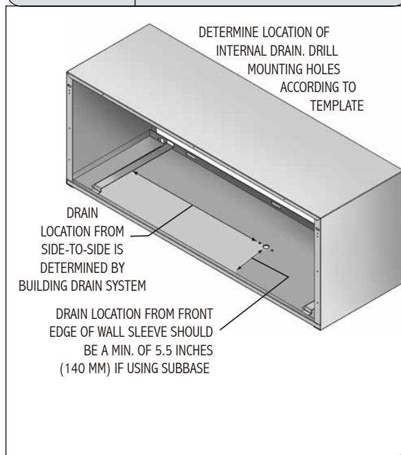
Figure 14 Internal Drain Installation
