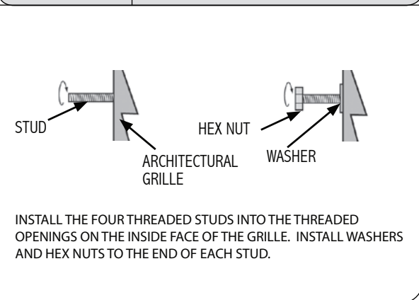
Figure 20 Threaded Stud Installation
