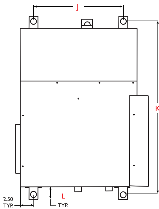
HANGING BRACKETS LOCATION
