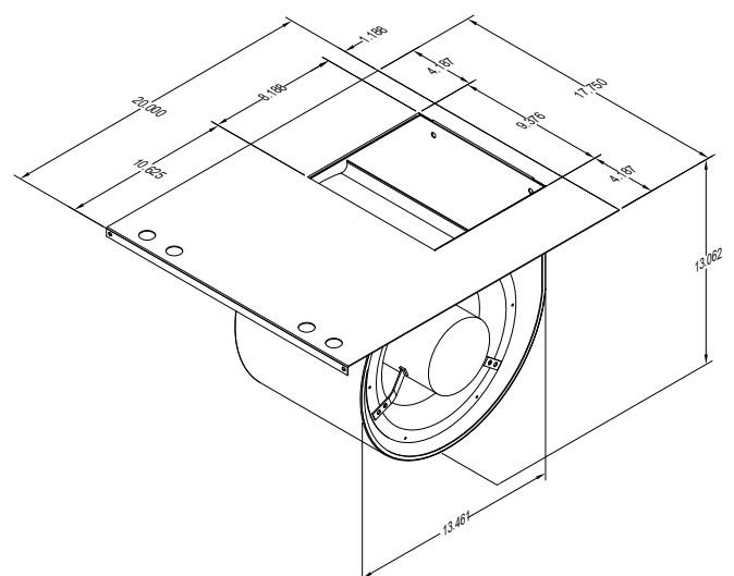
EZ18 Blower Assembly (Optional)
