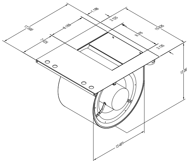
EZ12 / EZ15 Blower Assembly (Optional)
