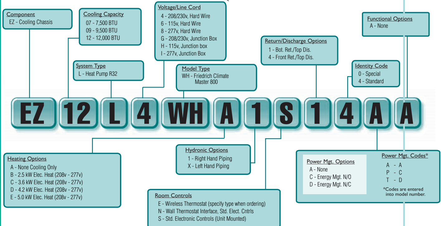
RIGHT HAND PIPING SHOWN
